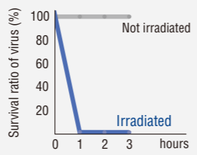
Test virus: Influenza virus (type A, H1N1) Test method: Virus inactivation test Test organisation: Japan Food Research Laboratories Result certificate: 10029107001-01 Results: The streamer unit removed 99% of the virus in one hour. A single type of virus was used in the simulation. The test showed the unit has a powerful effect on virus particles captured by the filter.
