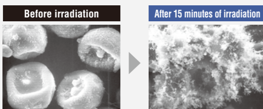
Cedar pollen was placed on an electrode of the streamer discharge unit and a picture was taken using an electron microscope after 15 minutes of discharge.
