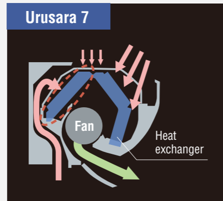
Air intake from both the top and bottom allows the back part of the heat exchanger to be used fully, resulting in higher energy efficiency.
