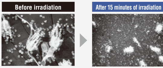
Cladosporium was placed on an electrode of the streamer discharge unit and a picture was taken using an electron microscope after 15 minutes of discharge.
