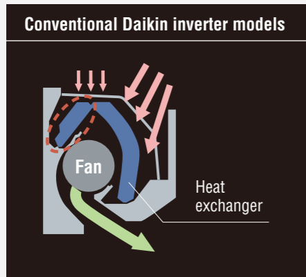
The back part of the heat exchanger is only partially used.
