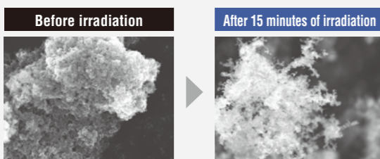
Diesel particles were placed on an electrode of the streamer discharge unit and a picture was taken using an electron microscope after 15 minutes of discharge.
